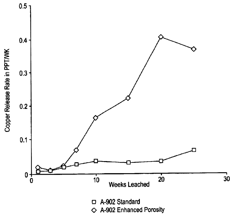
Effect of Outer Coating Porosity Enhancement
